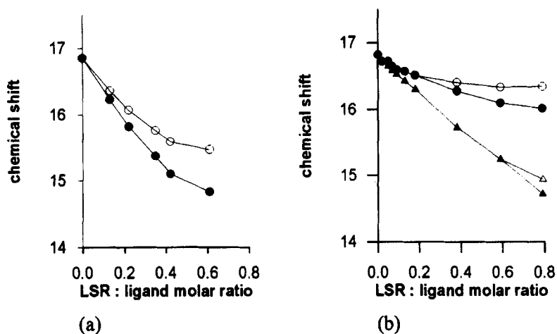
FIGURE 2 Plots of the \text{OCH}_2-\text{CH}_3 ^{13}\text{C} chemical shifts of ester 1 (a) and ester 2 (b) as a function of \text{Pr}(\text{hfc})_3 to substrate molar ratio
