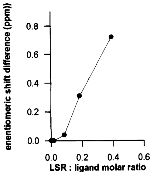
FIGURE 1 Plot of the enantiomeric shift difference \Delta\delta for \text{OCH}_3 carbon resonances of ester 7
