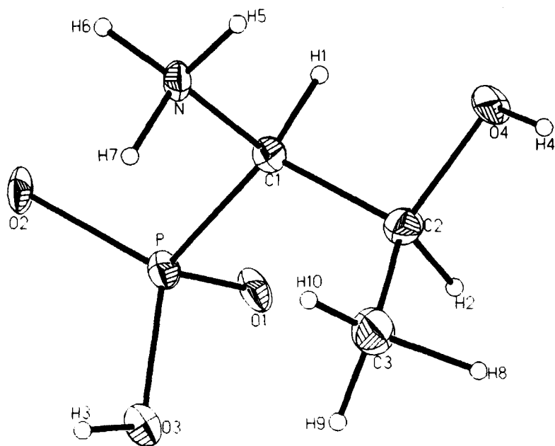
FIGURE 4 ORTEP [26] drawing of the (1R, 2S) diastereomer of 1-amino-2-hydroxypropane phosphonic acid racemate. Displacement ellipsoids are drawn at the 35% probability level
