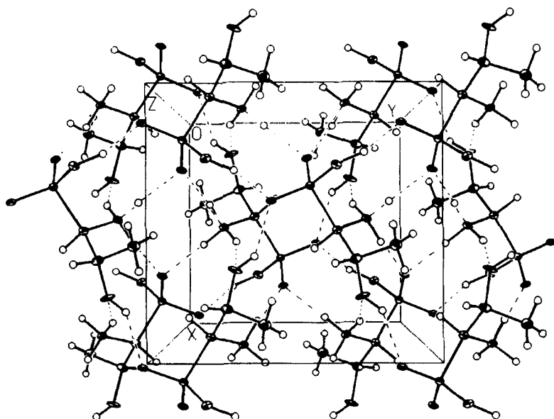
FIGURE 5 Packing diagram of molecules in crystal with hydrogen bonds indicated
