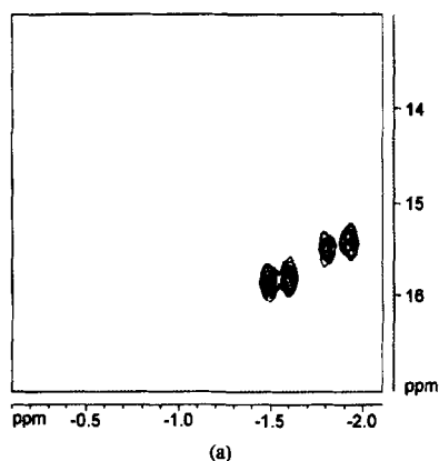
FIGURE 3 Expansion of \text{OCH}_2\text{-CH}_3 region of ^1\text{H}\text{-}^{13}\text{C} HMQC spectra at \text{Pr(hfc)}_3 : ester molar ratios of 0.39 (ester 1) – (a) and 0.79 (ester 2) – (b)
